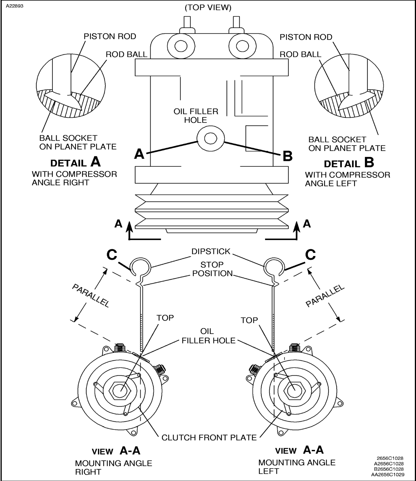
Figure 303 : Sheet 1 : R134a Compressor Oil Level Check
