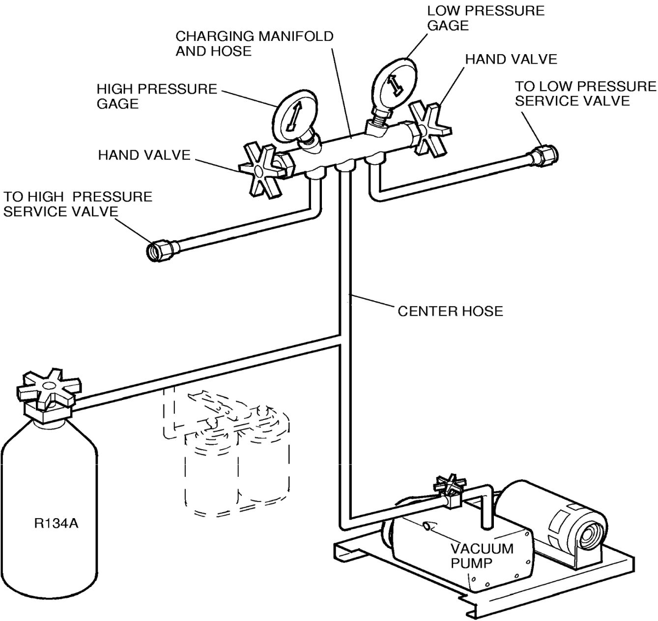
TYPICAL HOOKUP
